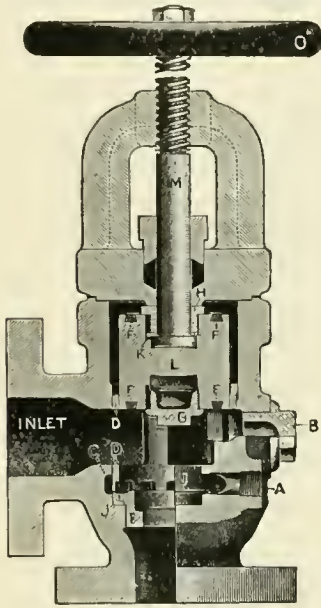
"DURO" BLOW-OFF VALVE.
